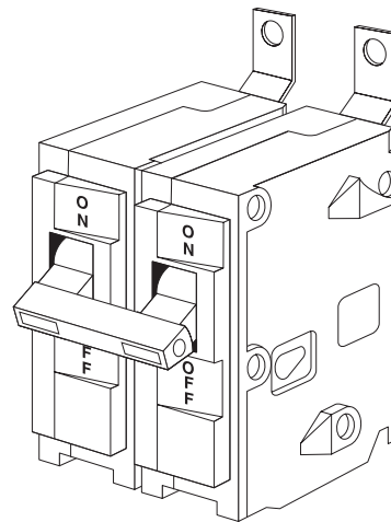
2-Pole Circuit Breaker Two Overcurrent Devices
