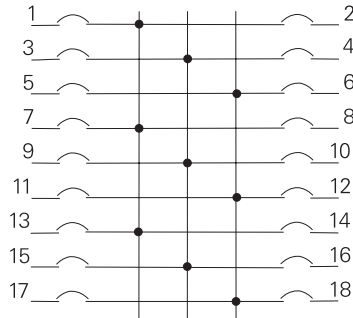
NEMA Numbering
