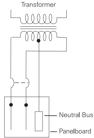
Overcurrent Protection Provided Ahead Of Panelboard
